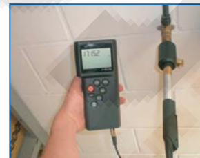
Pressure-tight moisture probe for measuring in compressed air
